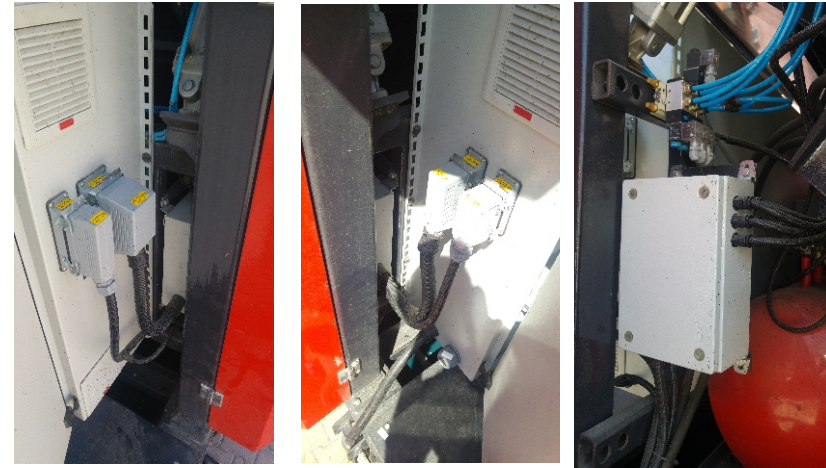
PLUG CONNECTION SYSTEM FOR EASY ASSEMBLY AND DISASSEMBLY.
